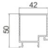
AC45-076 5mm Keel
