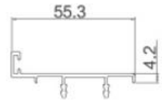
AC45-055 Unequal Double Door Capping
