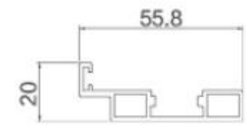
AC45-036 Unequal Double Door Covering
