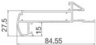
AC45-067 Casing
