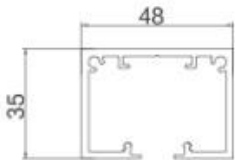
AC45-096 Hanging Rail
