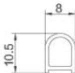
AC45-029 Grilles
