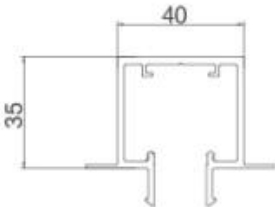
AC45-093 Hanging Rail
