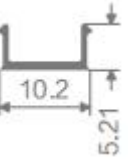
LED Cover Item No.: LJ-18020
