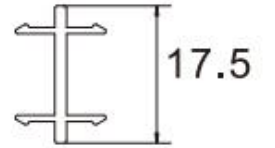
Top Rail Connector Item No.: LJ-8062 W/T: 0.8mm W/M: 0.12kg/m
