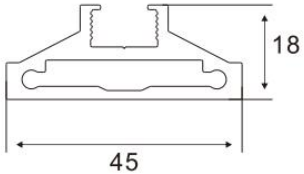
Door Frame Item No.:A-0170 W/T:2.5mm W/M:0.81kg/m
