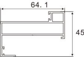
Door Jamb Item No.:A-0098 W/T:1.4mm W/M:0.868kg/m
