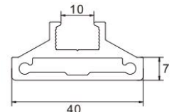
Door Frame Item No.:LJ-8007 W/T:2.5mm W/M:0.728kg/m
