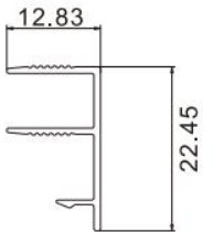
Door Back Cover Item No.:LJ-8046 W/T:0.9mm W/M:0.123kg/m
