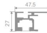
Side Column Item No.: LJ-18021
