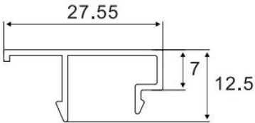
Partition Strip Cover Item No.:A-0114 W/T:1.0mm W/M:0.156kg/m
