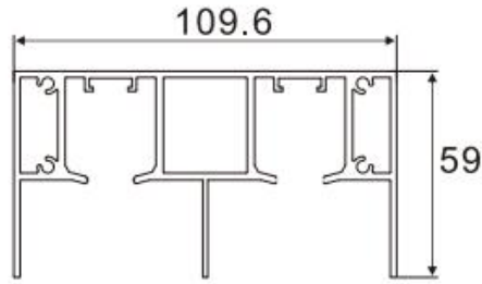
Hangig Rail Item No.:A-0094 W/T:1.8mm W/M:2.633kg/m
