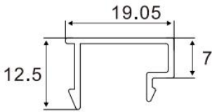
Partition Strip Cover Item No.:A-0113 W/T:1.0mm W/M:0.118kg/m
