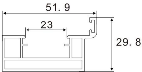
Door Frame Item No.:A-0117 W/T:1.4mm W/M:0.718kg/m
