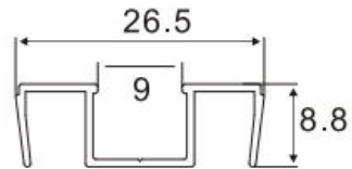
Conversion bar Item No.:A-0092 W/T:0.8mm W/M:0.172kg/m
