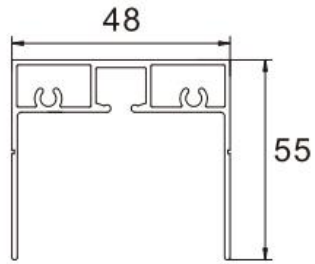
Top Rail Item No.: LJ-8001 W/T: 1.2mm W/M: 0.708kg/m
