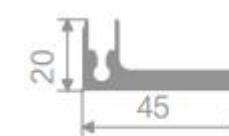
Shelf Rear/Side Baffle Item No.: LJ-18898
