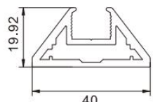
Door Frame Item No.:LJ-8088 W/T:2.2mm W/M:0.70kg/m
