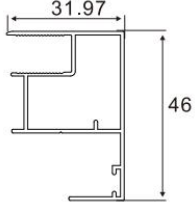
Door Back Cover Item No.:A-0101 W/T:1.2mm W/M:0.422kg/m
