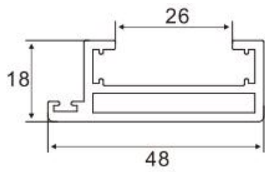
Door Frame Item No.:LJ-8011 W/T:2.0mm W/M:0.722kg/m
