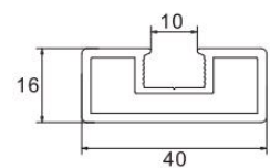
Door Frame Item No.:LJ-8013 W/T:2.0mm W/M:0.645kg/m
