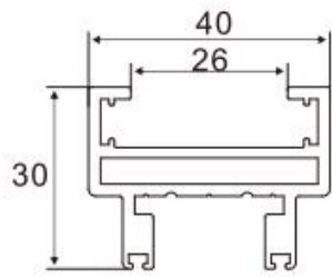
Door Frame Item No.:LJ-8012 W/T:2.0mm W/M:0.896kg/m
