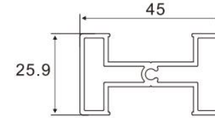
Separator Strip Item No.:A-0141 W/T:1.4mm W/M:0.72kg/m
