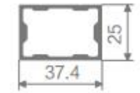
Side Crossbeam Item No.: LJ-18860
