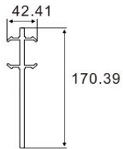
Top Rail Connector Item No.:A-0194 W/T:1.6mm W/M:0.233kg/m
