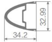
Ceiling Column A Item No.:LJ-20214
