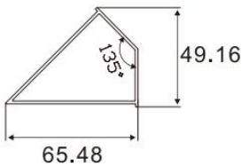
Corner Partition Strip Item No.:A-0119 W/T:1.4mm W/M:0.717kg/m
