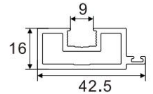
Corner Partition Strip
