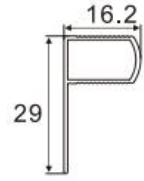
P Profile Item No.:A-0103 W/T:0.8mm W/M:0.146kg/m
