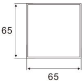
Corner Partition Strip Item No.:A-0118 W/T:1.4mm W/M:1.0kg/m
