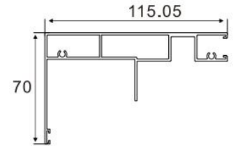
Top Rail Item No.:A-0193 W/T:1.4mm W/M:1.501kg/m
