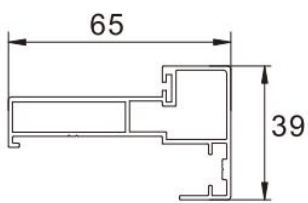
Door Jamb Item No.:LJ-8104 W/T:1.2mm W/M:0.81kg/m
