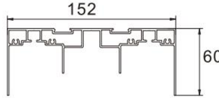
Top Rail Item No.: LJ-8003 W/T: 1.4mm W/M: 2.31kg/m
