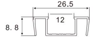
Conversion bar Item No.:A-0107 W/T:0.8mm W/M:0.13kg/m
