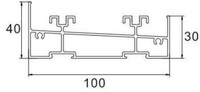
Floor Rail
