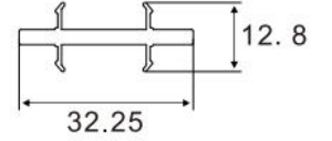
Hangig Rail Connector Item No.:A-0191 W/T:2.8mm W/M:0.301kg/m
