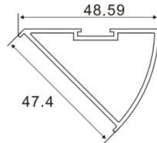
Corner Item No.:A-0142 W/T:1.4mm W/M:0.54kg/m
