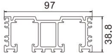
Hanging Rails Item No.: LJ-8036 W/T: 2.8mm W/M: 2.512kg/m
