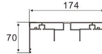
Top Rail Item No.:A-0120 W/T:1.4mm W/M:2.47kg/m
