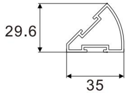
Corner Partition Strip
