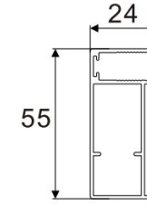
Door Jamb Cover
