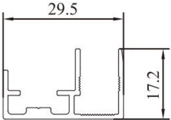
Door Back Cover Item No.: A-5006 W/T: 1.2mm W/M: 0.278kg/m
