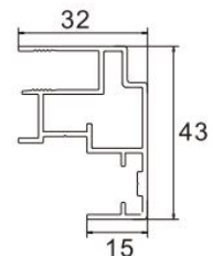
Door Back Cover Item No.:LJ-8047 W/T:1.2mm W/M:0.581kg/m
