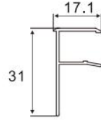
F Profile Item No.:A-0104 W/T:1.0mm W/M:0.157kg/m
