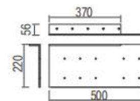
Shelf Rear/Side Baffle Item No.: LJ-18898
