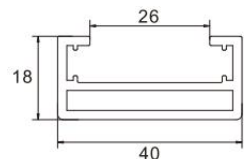
Rear Column Item No.:LJ-8010 W/T:2.0mm W/M:0.646kg/m
