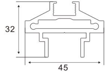
Door Frame Item No.:A-0172 W/T:2.5mm W/M:1.0kg/m
