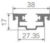
Ceiling Column B Item No.:LJ-20213
