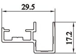
Door Back Cover Item No.: A-5007 W/T: 1.2mm W/M: 0.261kg/m
