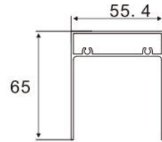
Top Rail Item No.:A-0165 W/T:1.4mm W/M:0.95kg/m
