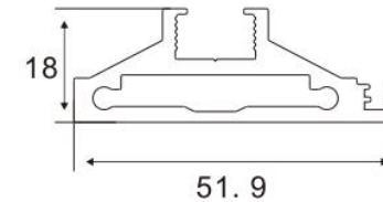
Door Frame Item No.:A-0171 W/T:2.5mm W/M:0.89kg/m
