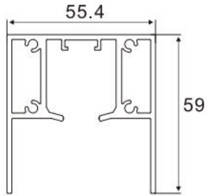
Hangig Rail Item No.:A-0095 W/T:1.8mm W/M:1.607kg/m
