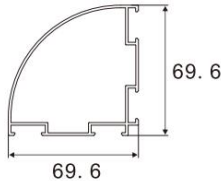
Corner Partition Strip Item No.:A-0116 W/T:1.4mm W/M:1.125kg/m
