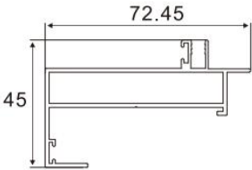
Door Jamb Item No.:A-0100 W/T:1.4mm W/M:0.832kg/m
