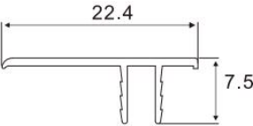
Door Jamb Cover Item No.:A-0106 W/T:0.9mm W/M:0.082kg/m
