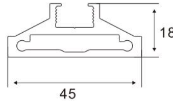
Door Frame Item No.:A-0170 W/T:2.5mm W/M:0.81kg/m
