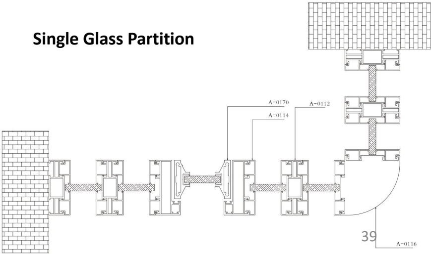
Corner Partition Strip Item No.:A-0116 W/T:1.4mm W/M:1.125kg/m
