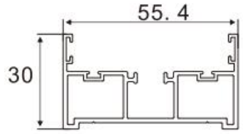
Door Jamb Item No.:A-0111 W/T:1.4mm W/M:0.744kg/m
