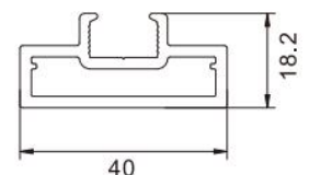
Door Frame Item No.:LJ-8093 W/T:2.2mm W/M:0.67kg/m
