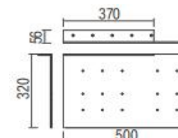
Shoes Shelf Baffle Item No.: LJ-19300
