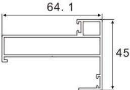
Door Jamb Item No.:A-0099 W/T:1.4mm W/M:0.868kg/m
