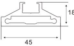
Door Frame Item No.:A-0170 W/T:2.5mm W/M:0.81kg/m
