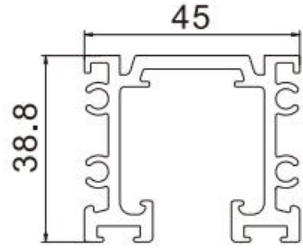
Hanging Rails Item No.: LJ-8035 W/T: 2.8mm W/M: 1.318kg/m
