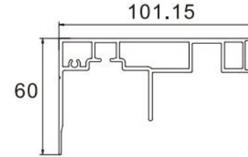
Top Rail Item No.: LJ-8061 W/T: 1.4mm W/M: 1.71kg/m
