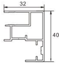
Door Back Cover Item No.:LJ-8106 W/T:1.2mm W/M:0.54kg/m
