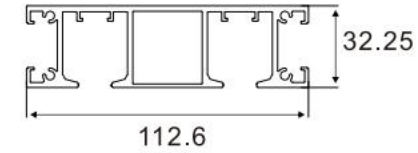
Hangig Rail Item No.:A-0190 W/T:2.2mm W/M:2.293kg/m
