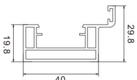
Door Frame Item No.:LJ-8065 W/T:1.2mm W/M:0.669kg/m
