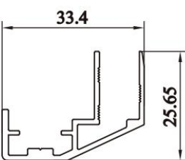
Door Back Cover Item No.: A-5008 W/T: 1.2mm W/M: 0.346kg/m
