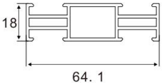
Partition Strip Item No.:A-0112 W/T:1.2mm W/M:0.914kg/m
