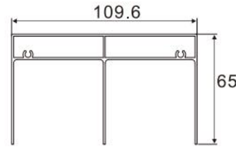
Top Rail Item No.:A-0096 W/T:1.4mm W/M:1.602kg/m
