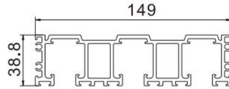
Hanging Rails Item No.: LJ-8037 W/T: 2.8mm W/M: 3.706kg/m
