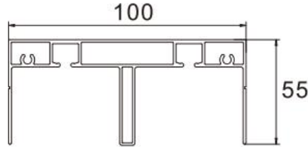
Top Rail Item No.: LJ-8002 W/T: 1.2mm W/M: 1.3kg/m
