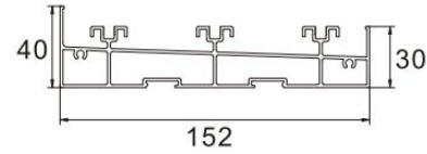
Floor Rail
